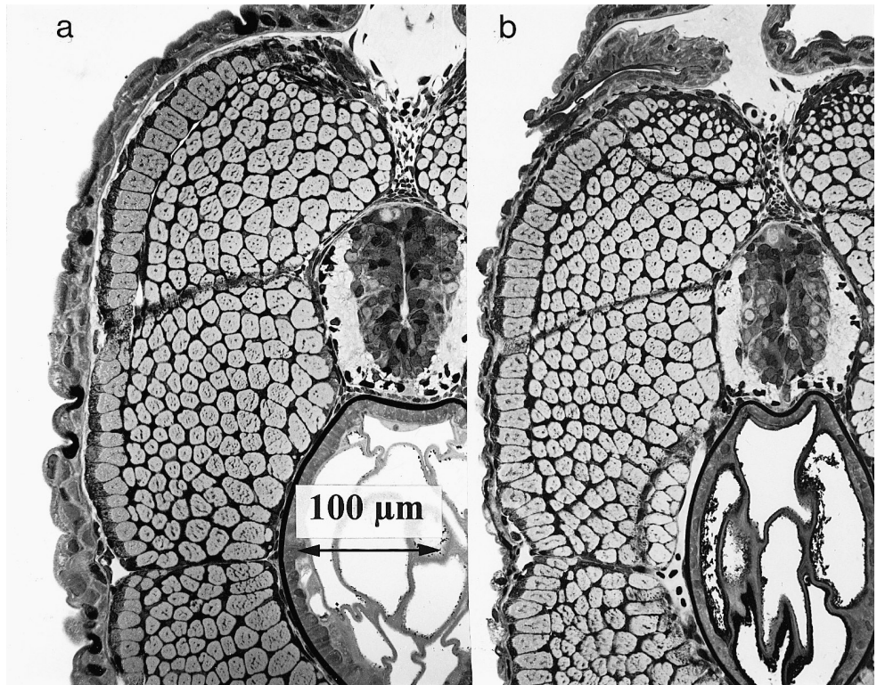
FIG. 1. Transverse sections of one quadrant of epaxial muscles in larvae of C. lavaretus , 1 day after hatching, reared at (a) 8° C or (b) 4° C. Fish were fixed in Karnovsky, semithin (3 µm) sections stained with periodic acid methamine silver (PAMS).
