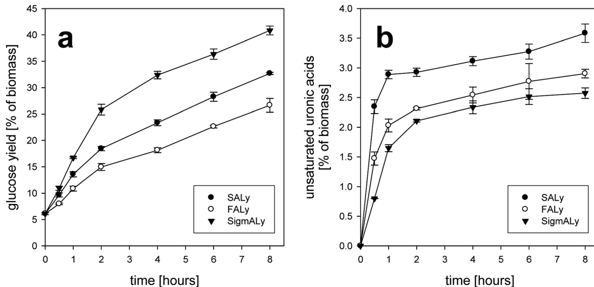
Fig. 4 (a) Glucose yields in % weight of dry biomass in response to enzymatic treatment; (b) alginate degradation products of unsaturated uronic acid residues in % by weight of dry biomass of refiner milled wet Laminaria digitata . Enzymatic saccharification with Cellic®CTec2 concentration of 10% v/w and alginate lyase (SALy, FALy and purchased lyase SigmALy) of 1% w/w over time with measurements at timepoints 0, 0.5, 1, 2, 4, 6 and 8 hours. Each data point represents the average value of independent duplicates; vertical bars indicate the standard deviation.
