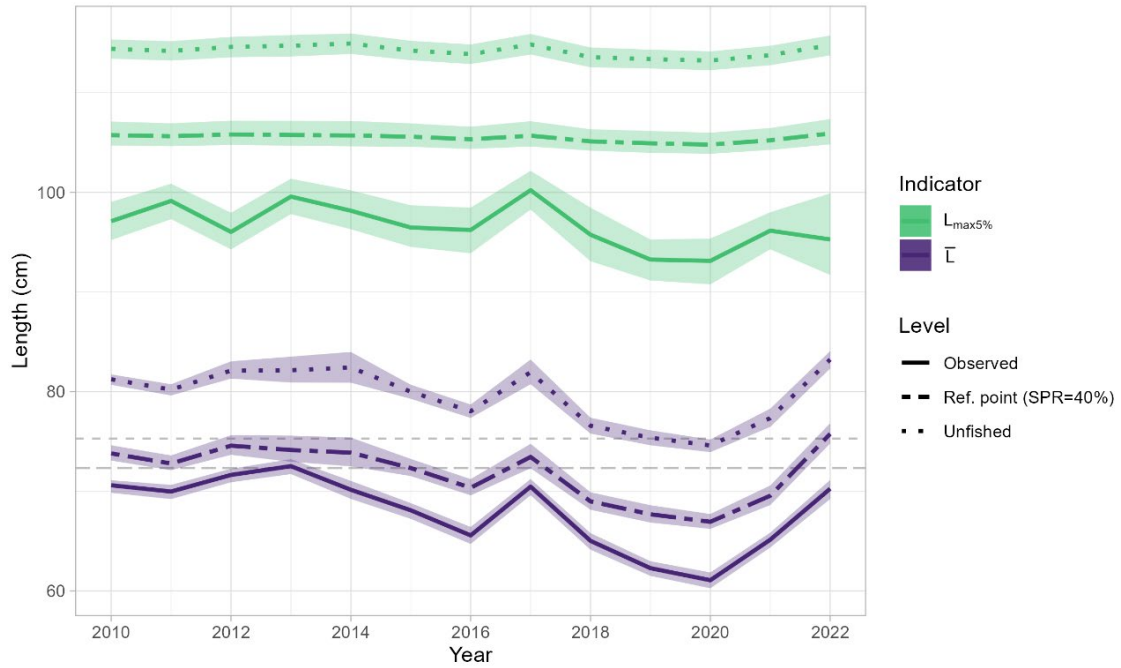
Figure 2.3.13. Length-based indicators L_{max5\%} and mean catch length ( \bar{L} ) in relation to their reference points (mean and 95%CI). The reference points were estimated using the LBSPR simulation model together with the stochastic parameters detailed in Table 2.3.1 (mortality scenario following Lorenzen, 1996) and SPRs of 40% and 100% (unfished).
