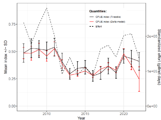
Figure 6. Standardized CPUE (kg per gillnet day) +/- SD (solid black line with error bars for the original Tweedie model, and solid red line with error bars for the new delta model) and the corresponding standardized effort (dash line) for anglerfish based on the data from the Norwegian coastal reference fleet in ICES Subarea 2a, from vessels targeting anglerfish with large-meshed gillnets.
