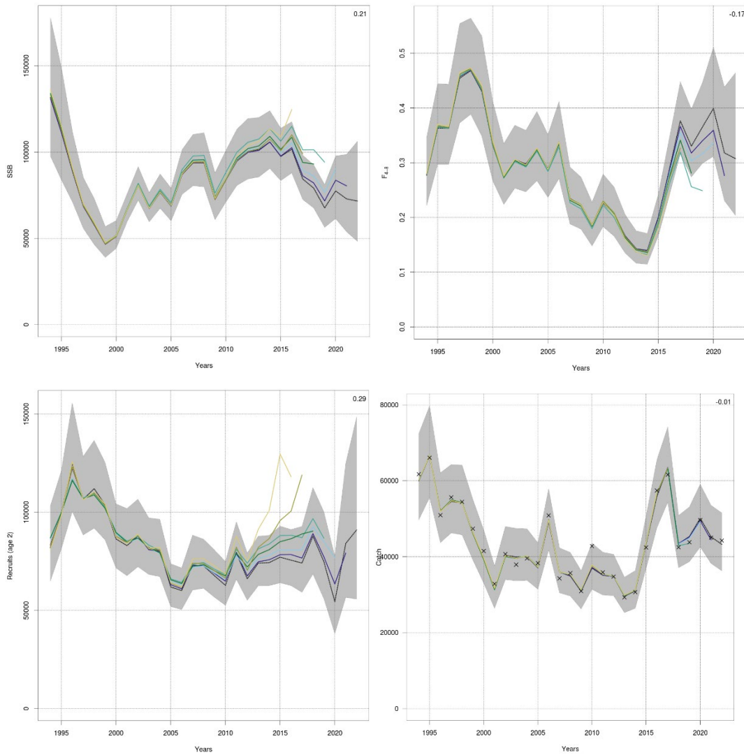
Figure 2.2.9. Northern Norwegian coastal cod. Northern Norwegian coastal cod. 5-year retrospective peel: a) SSB, b) F_{bar} , c) recruitment, and d) catch. The Mohn's rho value (5-year average retrospective bias) is indicated in the upper right corner of each panel.
