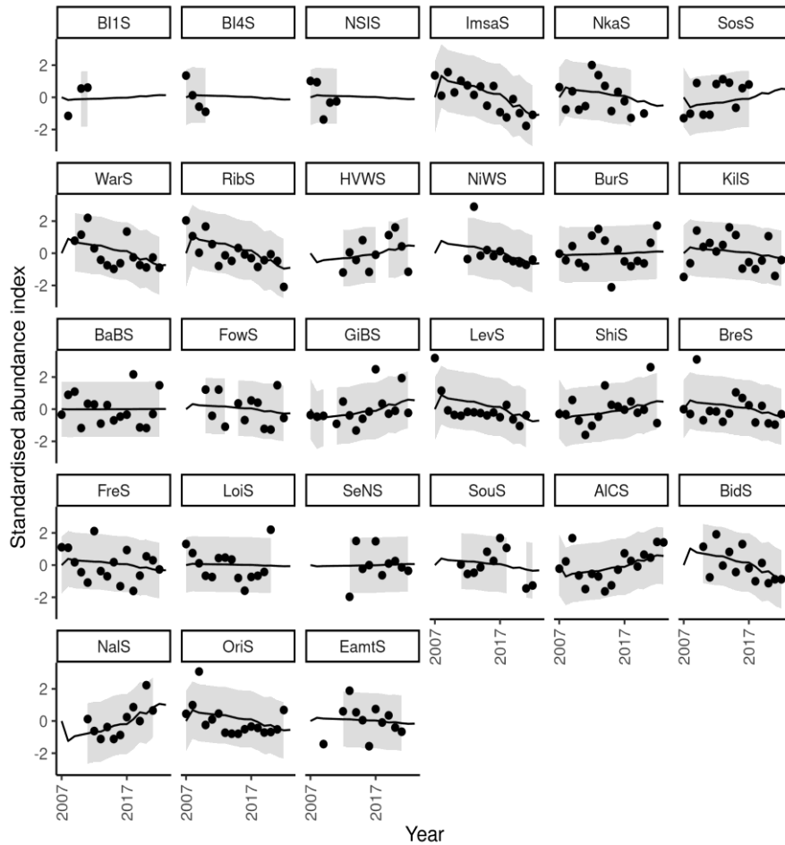
Figure 2.37 DFA fits to time series using the data set since 2007. Points = raw data, black line = DFA fit, grey zone = confidence interval.
