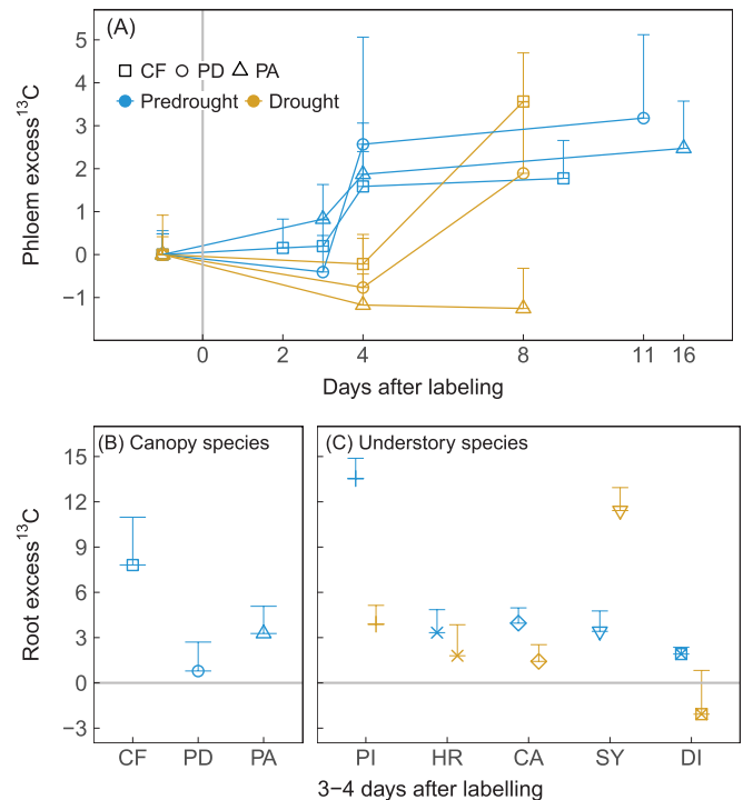
Fig. 5. Impacts of drought on the transport of recent photosynthates. Temporal changes of the ^{13}\text{C} label (the excess ^{13}\text{C} relative to the pre-labeling ^{13}\text{C} values in atom %) in soluble carbon in the stem phloem (A) and roots (B, C) under pre-drought and drought conditions ( n=3 or 4 plants per species). Stem phloem data are shown for the three canopy species, namely Clitoria fairchildiana (CF), Phytolacca dioica (PD), and Pachira aquatica (PA). Root data are shown for the canopy species, as well as understorey species Piper auritum (PI), Hibiscus rosa sinensis (HR), Calathea sp. (CA), Syngonium sp. (SY), and Dieffenbachia sp. (DI) within 4 d after labeling. Note that root ^{13}\text{C} data are missing for the canopy species under drought conditions due to sample loss during the shipping process. For clarity, all values were multiplied by 1000. Error bars represent the coefficient of variation for pre-labeling (day -1) and propagated SEs after labeling.
