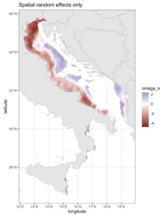
Figure 4.1.8.3. Spatial random effects.
