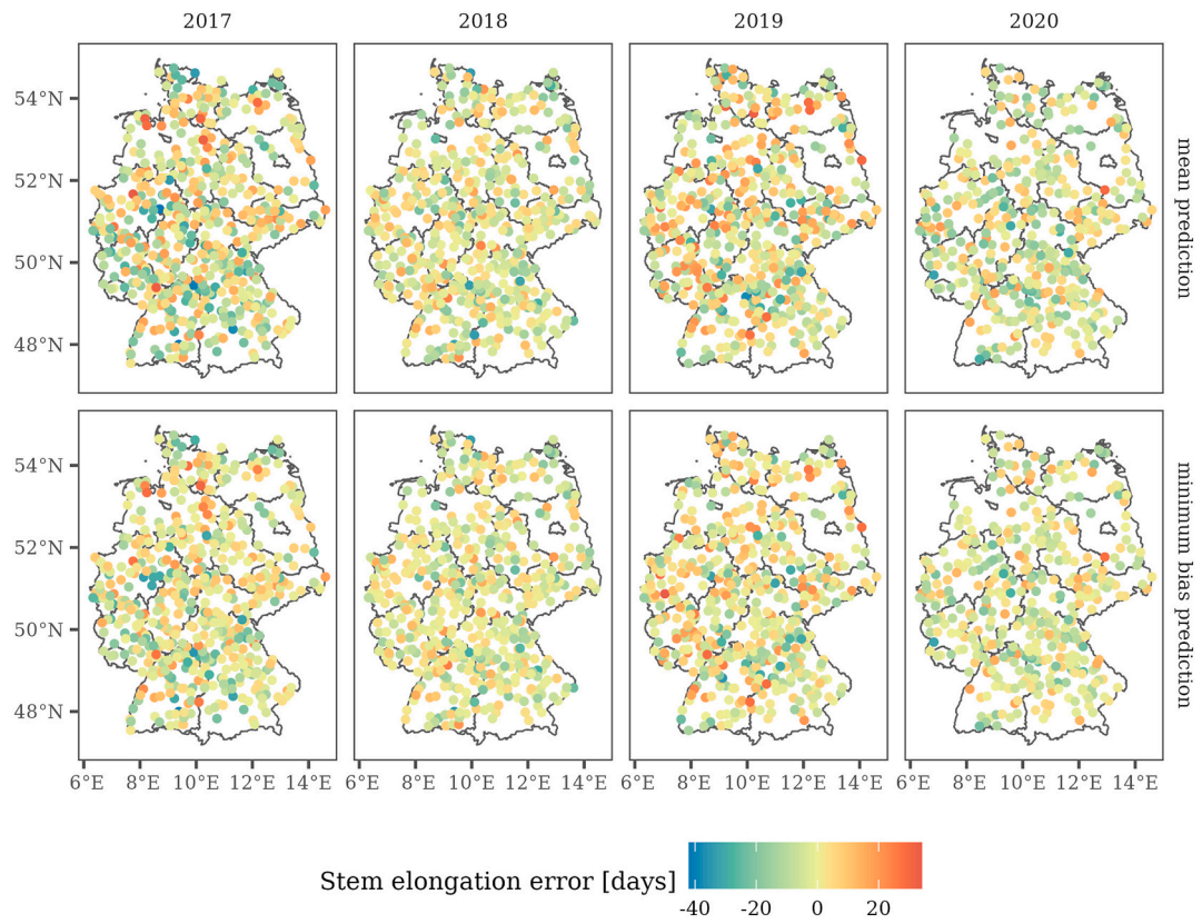
Fig. A9. Difference of predictions and reference dates for the stem elongation of winter wheat in Germany between 2017 and 2020.
