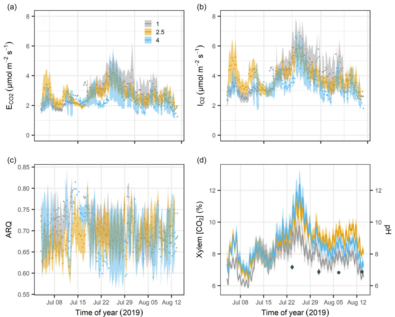
FIGURE 2 (a) CO 2 efflux ( E_{\text{CO}_2} ), (b) O 2 influx ( I_{\text{O}_2} ), (c) the apparent respiratory quotient (ARQ; E_{\text{CO}_2}/I_{\text{O}_2} ) and (d) internal xylem [CO 2 ] at 1, 2.5 and 4 m height from 4 July to 14 August 2019. Sap pH (d, black dots) was measured from twigs ( n = 3 ). [Color figure can be viewed at wileyonlinelibrary.com ]
