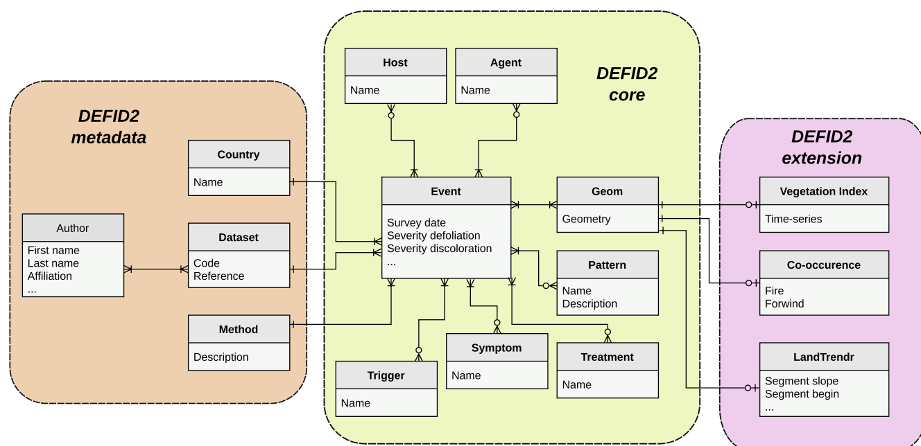
FIGURE 1 Simplified entity relation diagram (ERD) of the DEFID2 database.
