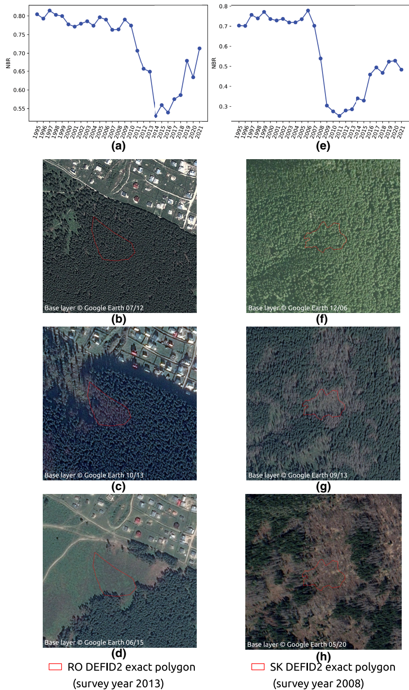
FIGURE 8 Examples of satellite-based forest dynamics in areas affected by insect disturbances. Annual changes in satellite normalized burn ratio index (NBR) over forest areas located nearby the town of Mironu in Suceava district, Romania (RO) (a), and nearby the town of Podbanské in Tatra Mountains in Poprad district, Slovakia (SK) (e), affected by insect outbreaks surveyed in 2013 and 2008, respectively. Satellite imagery shown in (b–d) and in (f–h) clearly displays the changes in forest cover during the outbreaks for the two case studies considered.
