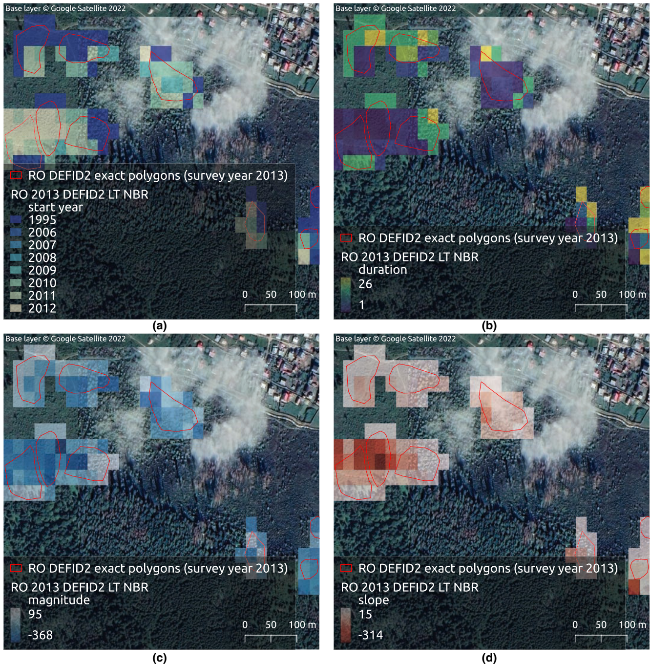
FIGURE 9 Example of four key metrics describing the spectral trajectories identified in the DEFID2 disturbance records as retrieved using the LandTrendr algorithm. The outbreak occurred near the town of Mironu in Suceava district, Romania (RO) and was surveyed in 2013 (red lines on the map). Displayed metrics are start year (a), duration (years) (b), magnitude of change (c), and slope of the trends (d) measured over the DEFID2 records.
