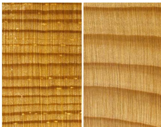
Figure 4: Macroscopic structure of softwoods. (left): transverse plane of spruce with the occurrence of resin canals. (right): transverse plane of white fir without resin canals
