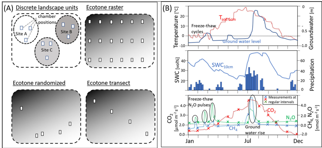
FIGURE 1 (A) Overview of different spatial layout types of chamber positions within different spatial structures (adapted from figure 1 of the full Guideline, Fiedler et al., 2022). (B) Exemplary (fictional) temporal evolution of (top) soil temperature and ground water, (middle) precipitation and soil water content (SWC) and (bottom) fluxes of CO 2 , N 2 O and CH 4 .
