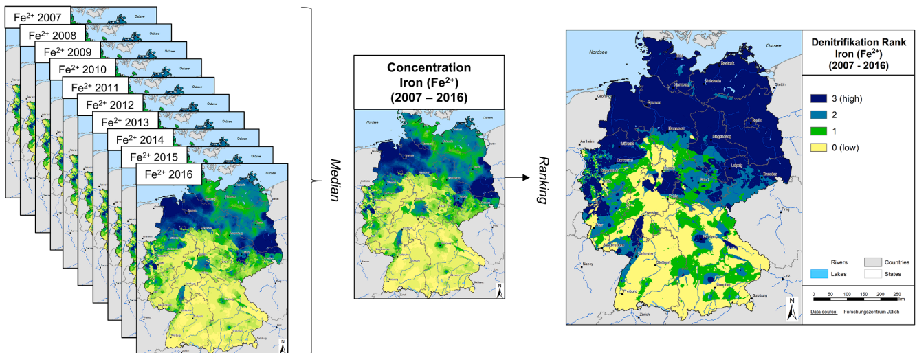
Fig. 5. Exemplary result of the procedure for median averaging from 10 interpolated yearly Fe^{2+} concentrations (2007 – 2016) and successive ranking according to the redox indication classes specified in Table 1.
