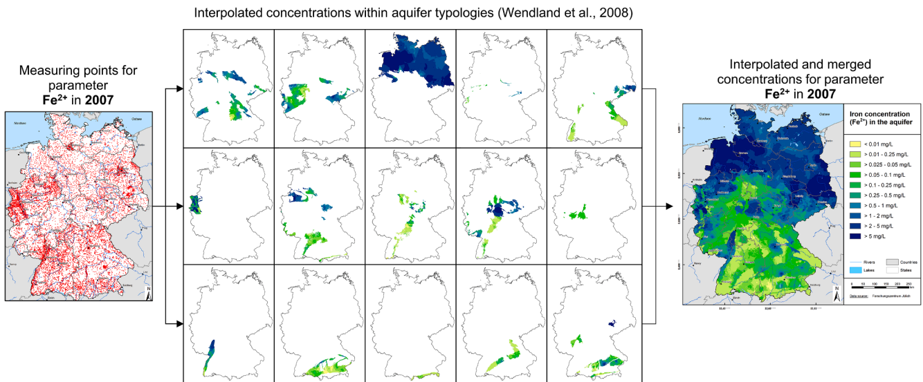
Fig. 4. Exemplary result of the interpolating procedure of groundwater quality parameters for Fe^{2+} measurements in 2007.
