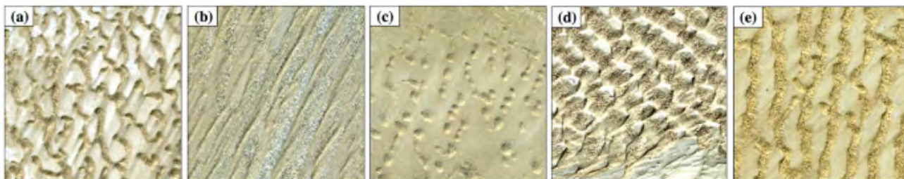
Figure 12. Geomorphic structural diversity, monitored with remote sensing technology. Examples of dune-field landscape patterns on remotely sensed data. (a) Barchan dunes, (b) linear dunes, (c) dome dunes, (d) reticulate dunes, and (e) longitudinal dunes (reprinted with permission from Zeng et al. [117], 2021, Elsevier. license no. 5176660806321).
