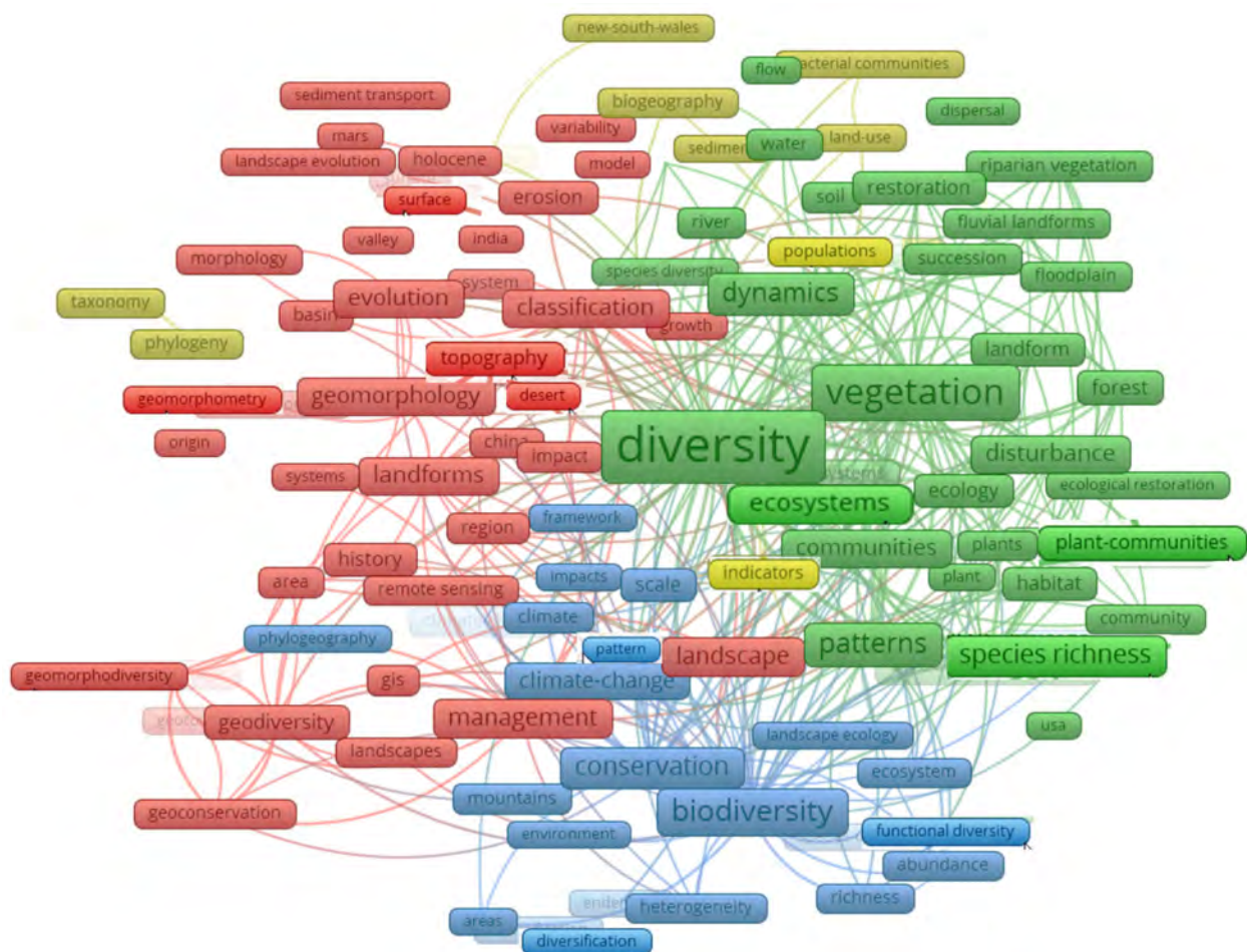
Figure 19. Keywords and their co-occurrence in a bibliographic search in the Web of Science, with the topics: “geomorphodiversity” or “geomorphological diversity” or “landform diversity”; date of analysis, April 2022, finding 653 papers and around 100 keywords.
