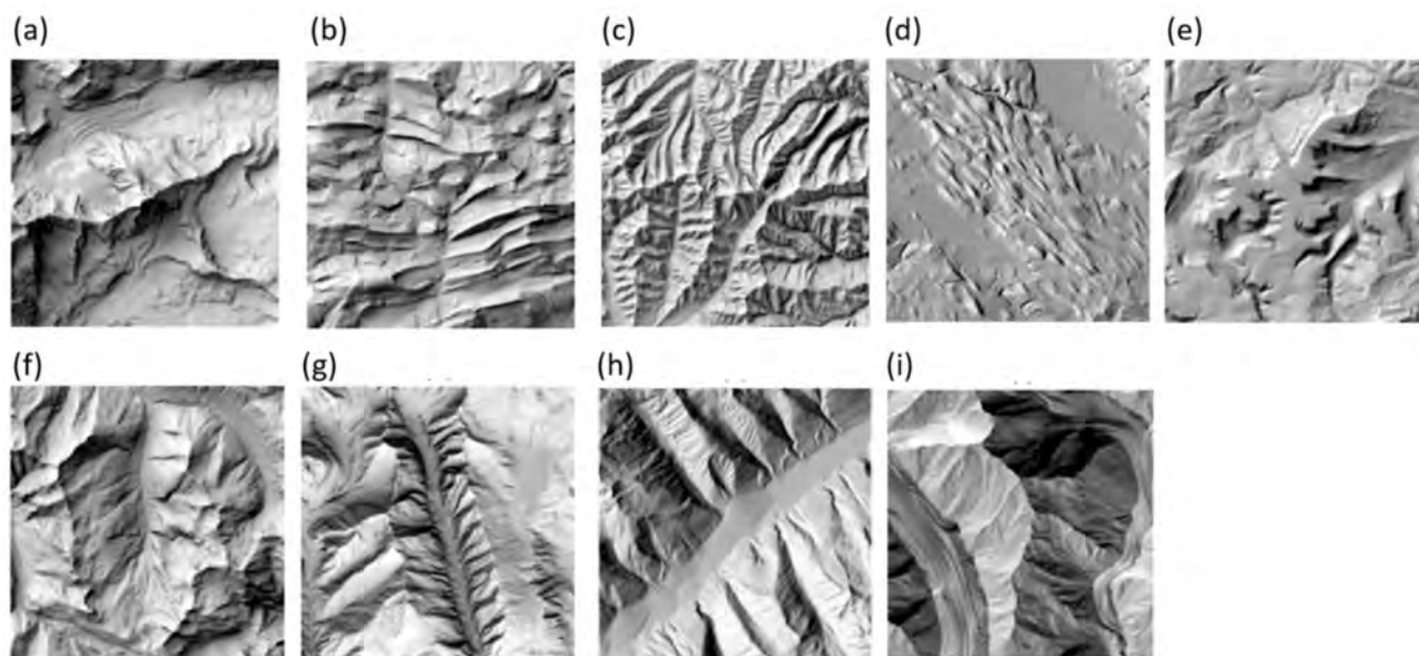
Figure 13. Geomorphic taxonomic diversity using RS. The most suitable relief shading methods per landform based on the survey results: the clear sky model method for (a) block mountains; (b) folded mountains; (c) mountains formed by erosion processes; (d) cluster shading for drumlins; (e) plateaus; and (f) V-shaped valleys; (g) clear sky model with custom illumination (here, S) for U-shaped valleys; (h) standard hill-shading with custom illumination (here, W) for alluvial fans; and (i) aspect shading for glaciers (from Farmakis-Serebryakova et al. [98]).
