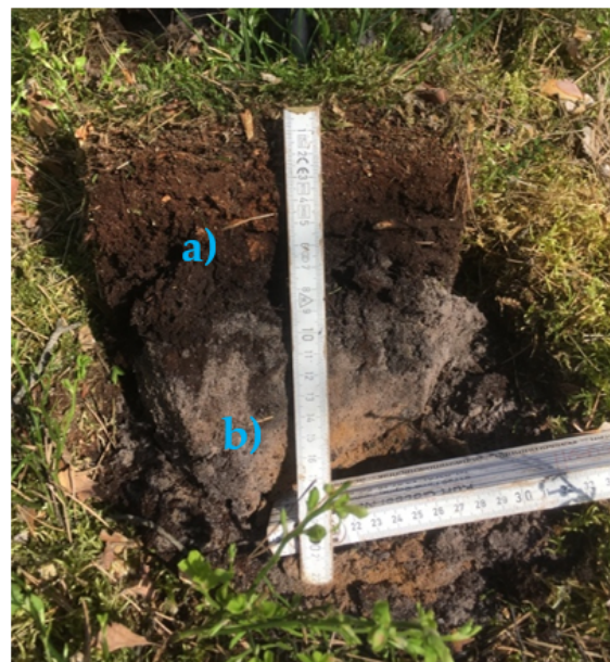
Figure 2. Exemplary representation of a sampled pine forest (left) with the top soil (a) and upper mineral soil (b).
