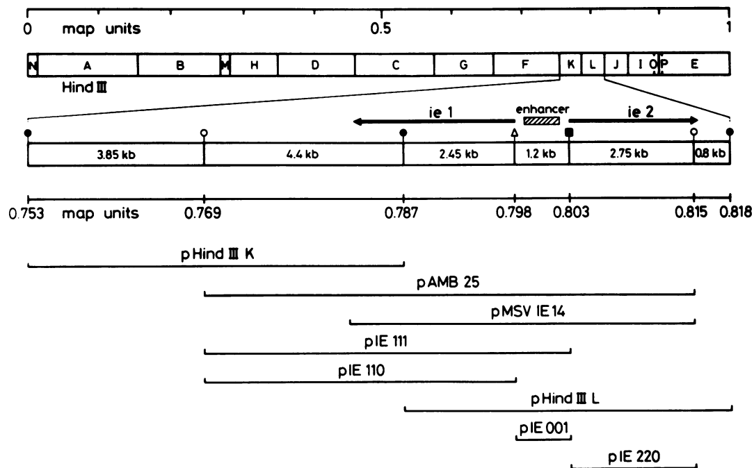
FIG. 1. Physical map of the MCMV genome. The location of the Hind III cleavage sites is shown. The region encoding the 2.75-kb transcript of ie1 and the 1.75-kb transcript of ie2 separated by the long >700-base-pair enhancer sequence is expanded. The plasmid pMSV-IE14, which contains a 7.8-kb MCMV DNA fragment, was used for the introduction of ie1 into L cells. The 10.8-kb Bam HI fragment (plasmid pAMB25) was used as a probe to detect MCMV sequences inserted into cellular DNA and mRNA transcribed in L cells. The other plasmids were used in transient assays to monitor the trans -activating function of the IE gene products. The arrows indicate the start and the direction of transcription of the IE genes. Symbols: ●, Hind III; Δ, Dra I; ■, Hpa I; ○, Bam HI.
