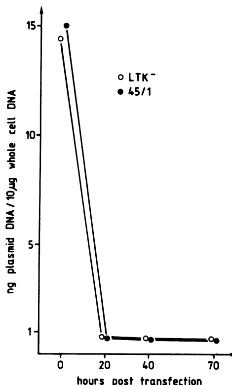
FIG. 4. Stability of transfected plasmid DNA in L cells and 45/1 cells which express pp89 of MCMV. Cells were transfected with 10 \mu g of pSRM2-CAT, and whole cell DNA was extracted at various times. The time point after removal of the calcium phosphate precipitate was taken as the sample at 0 h. Two replicate plates were extracted. Total DNA (10 \mu g) was blotted onto nitrocellulose and hybridized to a [ 32 P]cRNA probe specific for the CAT gene. The amount of plasmid DNA in cells was determined by autoradiography using a standard dilution of plasmid DNA. The results were corrected for the number of cells per culture dish determined at 0 h to exclude the effect of different growth rates. Four replicate determinations were carried out at 40 h; two were used for the determination of CAT activity. The chloramphenicol conversion rate by extracts from L cells was 46% and from 45/1 cells was 45%.
