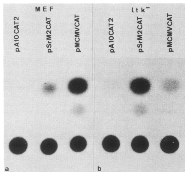
FIG. 6. Cell-specific activity of the MCMV enhancer. DNA of plasmids containing the CAT gene construct and the SV40 promoter alone (pA10-CAT2) or, in addition, the MSV long terminal repeat enhancer (pSrM2-CAT) or the MCMV enhancer sequences (pMCMV-CAT) were transfected into MEF (a) or L cells (b). For transfection of MEF, 20 \mu g of calcium phosphate-precipitated DNA was used, and Ltk - cells were transfected with 5 \mu g of DNA by the DEAE-dextran precipitate technique. Cell extracts were prepared 40 h later and assayed for CAT activity.
