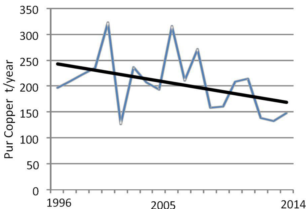
Figure 1: Estimated amounts of pure copper [t] based on the sales of copper pesticides in Germany from 1996 to 2014, EXEL trend line.
