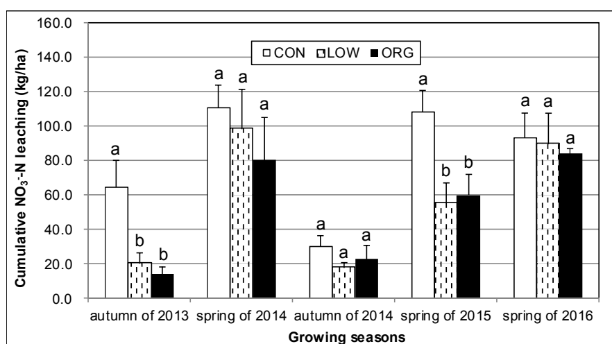
Figure 2. Cumulative NO 3 - -N leaching losses in three production systems
