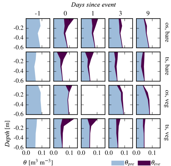
Figure 3. Mean daily soil water content \theta along soil depth separated into pre-event soil water content \theta_{pre} and infiltrated event soil water content \theta_{eve} . Observations are displayed for plots under bare soil (bare) or vegetation cover (veg) at open sites between tree crowns (os) and shaded sites beneath tree crowns (ts). Numbers at the top mark days since the watering event. Uncertainties for soil moisture observations during the experiment amount on average to 2.3 % vol. propagated from the observations. Event water partitioning for day 1 on open, vegetated plots needed to be omitted due to inadequate field data quality.
