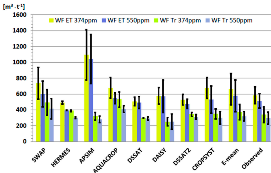
Figure 7. Water footprints of winter wheat calculated from simulations of different models for ambient (374 ppm) and elevated (550 ppm) CO 2 concentrations of the FACE experiment at Braunschweig/Germany. Error bars of the model results and observations show inter-annual variability, error bars of the ensemble mean the inter-model variability. “Observed” is calculated from simulated ET and Tr and observed yields.
