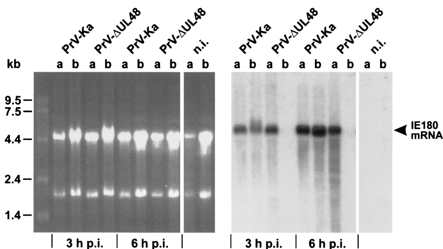
FIG. 7. Induction of immediate-early gene expression by the UL48 protein of PrV. RK-UL48 (lanes a) and normal RK13 cells (lanes b) were infected with either PrV-Ka or PrV- \Delta UL48 and incubated in the presence of cycloheximide for 3 or 6 h. Total RNA of infected and noninfected (n.i.) cells was separated in a denaturing agarose gel (left) and transferred to a nylon membrane. The blot was hybridized with a probe specific for the major immediate-early transcript of PrV (IE180 mRNA; right).
