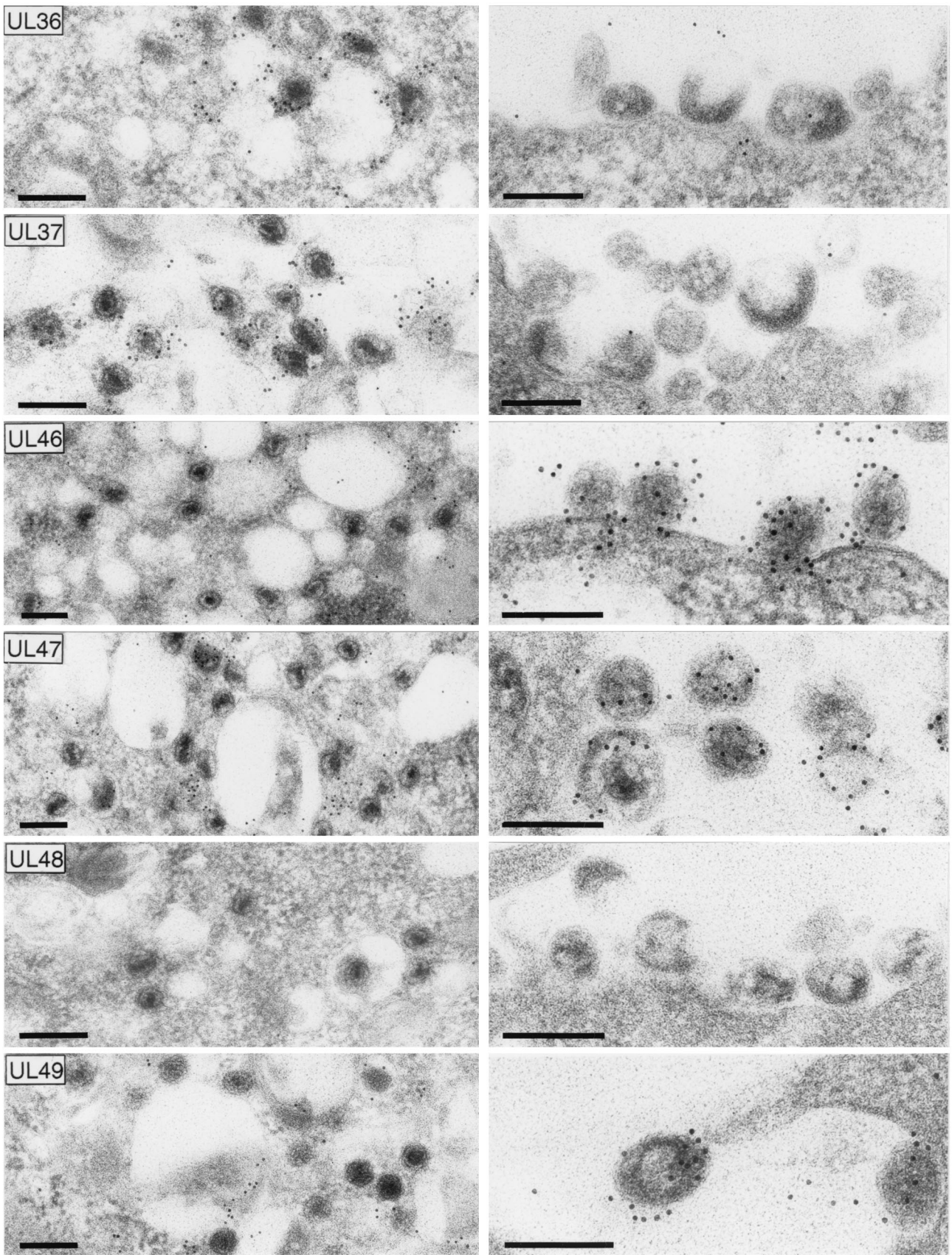
FIG. 9. Association of tegument proteins with cytoplasmic nucleocapsids (left panels) and released capsidless particles (right panels) of PrV-ΔUL48. Infected RK13 cells (see Fig. 8) were embedded for immunoelectron microscopy, and ultrathin sections were incubated with monospecific rabbit sera against the UL36, UL37, UL46, UL47, UL48, and UL49 gene products and 10-nm gold-tagged secondary anti-rabbit antibodies. Bars, 200 nm.
