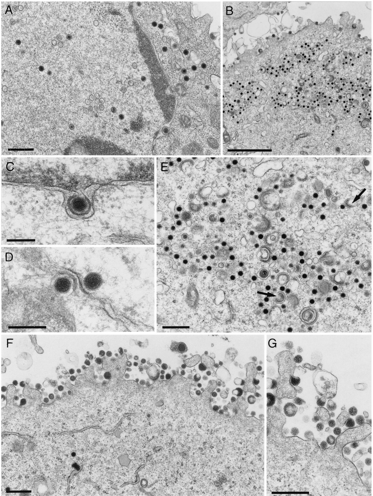
FIG. 8. Virion morphogenesis of PrV- \Delta UL48. For electron microscopy, RK13 cells were fixed and embedded 14 h after infection with phenotypically complemented PrV- \Delta UL48 (MOI, 1). The counterstained ultrathin sections showed all stages of intranuclear capsid maturation (A), as well as primary envelopment (C) and de-envelopment (D). However, nonenveloped nucleocapsids accumulated in the cytoplasm (B and E), and numerous capsidless particles were formed (E, arrows) and released from the cells (F and G). Bars, 500 nm (A), 2 \mu m (B), 200 nm (C and D), and 500 nm (E to G).
