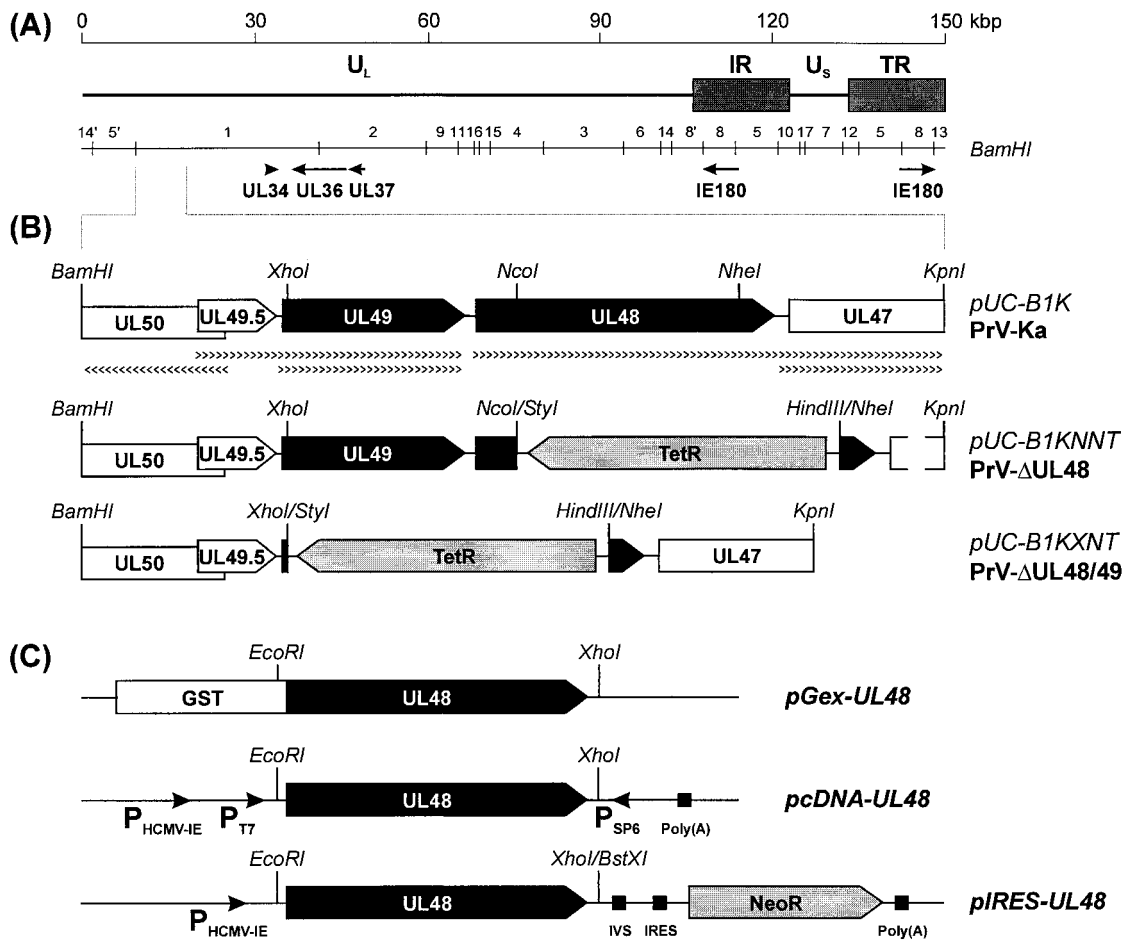
FIG. 1. Generation of plasmids and virus mutants. (A) Schematic map of the PrV genome, which consists of a unique long (U L ) region and a unique short (U S ) region, which is bracketed by inverted-repeat sequences (IR and TR). The positions of Bam HI restriction fragments and of genes relevant for this study are indicated. (B) Enlarged map of a plasmid-cloned DNA fragment of PrV-Ka (pUC-B1K) including relevant restriction sites. Transcriptional organization of genes UL50 to UL47 (pointed rectangles) is also shown. Deletion mutants PrV-ΔUL48 and PrV-ΔUL48/49 contain the tetracycline resistance gene (encoding TetR), since they were generated by mutagenesis of an infectious clone of PrV-Ka with plasmid pUC-B1KNTT or pUCB1KXNT in E. coli . (C) A UL48-GST fusion protein was expressed from pGex-UL48, whereas pcDNA-UL48 was used for in vitro transcription from the bacteriophage T7 and SP6 promoters (P T7 , P SP6 ) and subsequent in vitro translation. Plasmid pIRES-UL48 contains a bicistronic transcription unit of the UL48 gene and the neomycin resistance gene (NeoR), which are separated by an intron (IVS) and an internal ribosomal entry site (IRES) and which are flanked by the human cytomegalovirus immediate-early promoter (P HCMV-IE ) and a polyadenylation signal [Poly(A)].
